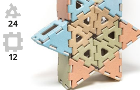
3D Star*
