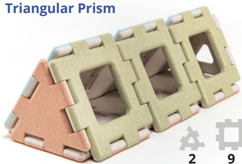
Kepler Matrix
