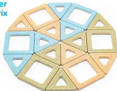
Cuboctahedron
